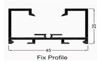
Taiton Tavic Fixed Glazed Partition Fix Profile Size 25mm x 45mm Length 3.0 Mtr
