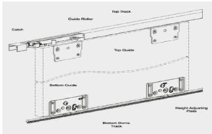
Ebco Aluminium Profile Hi Slide-90 Dome Track (FITTINGS)
