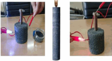
Electrically Conductive Concrete (ECC)
