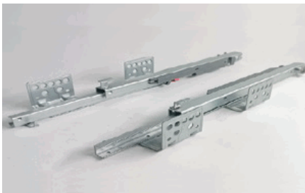
Ebco Concealed Drawer Slides Partial Extension 2 Size- 385mm
