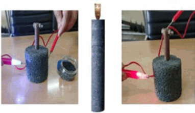
Electrically Conductive Concrete (ECC)
