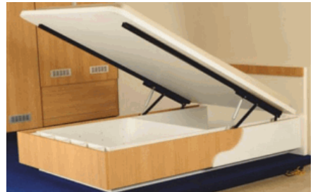
Ebco Pro Lift Gas Lift 750N
